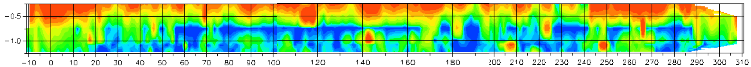
Resistivity data in YOZ plan for X:24.8
